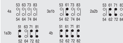
Contact Configuration
